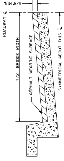
DETAIL B BRIDGE HALF TYPICAL SECTION
